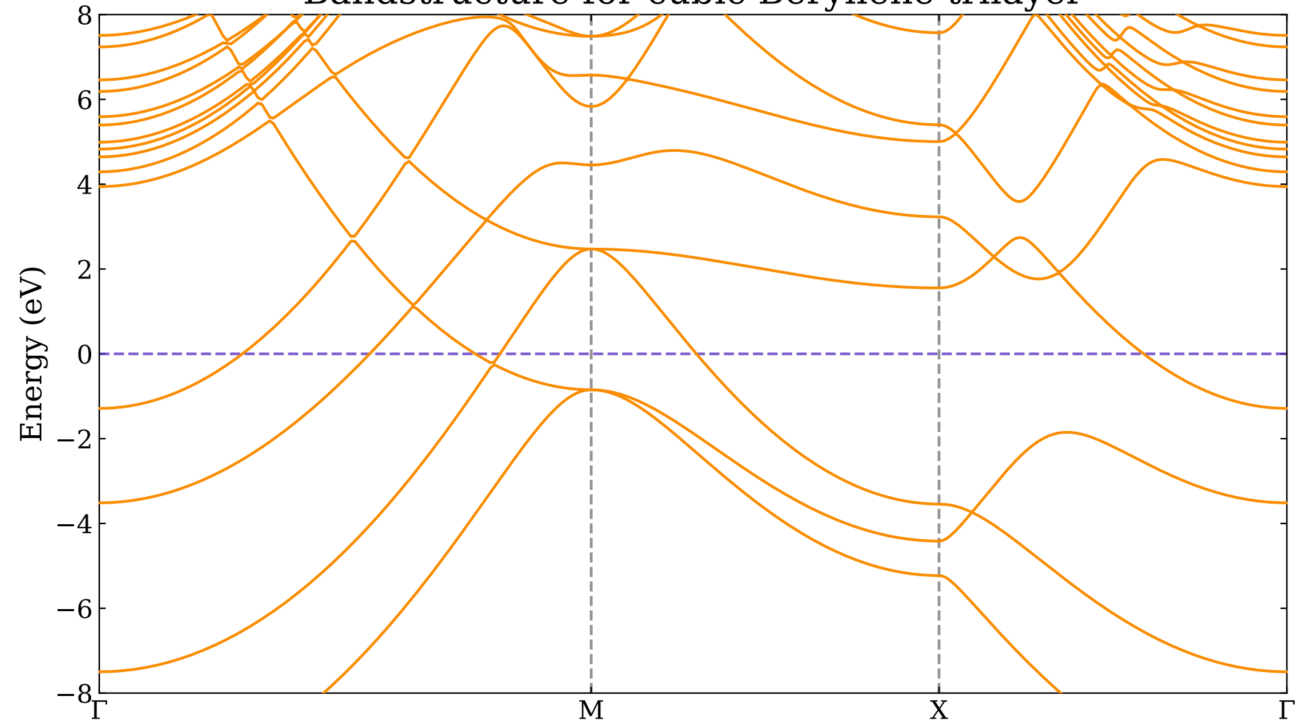
Bandstructure for cubic Beryllene trilayer
