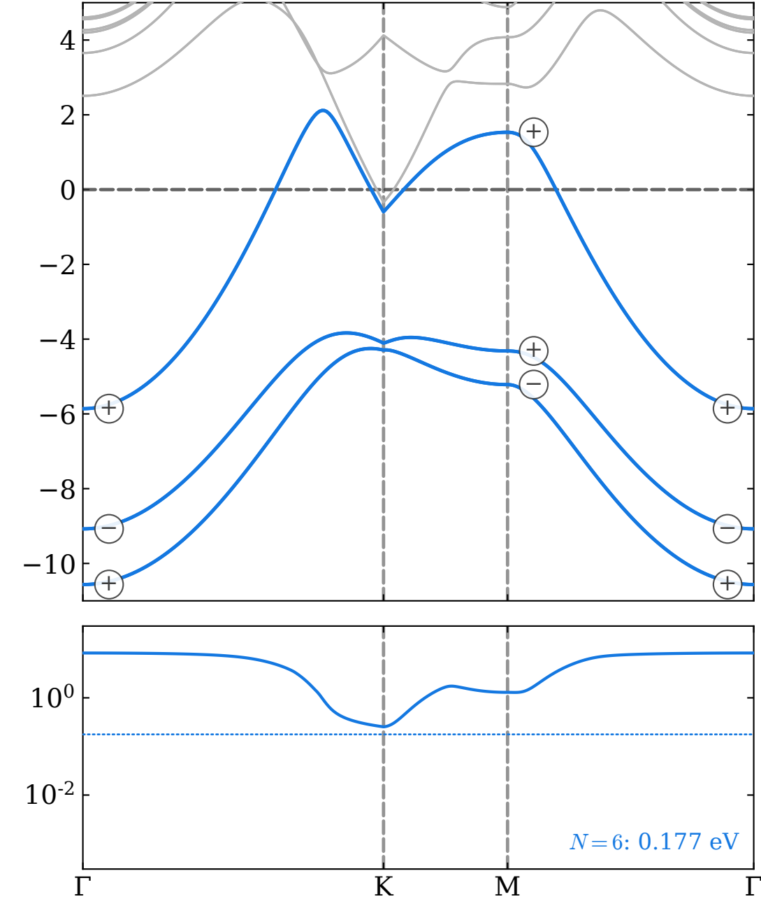
(c) 2H- \beta -beryllene: \nu = 0 N = 6
