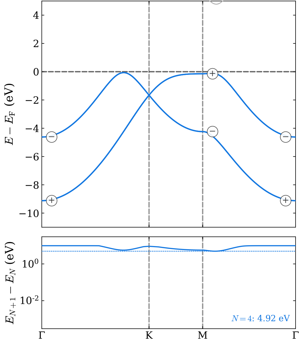
(a) 2H- \alpha -beryllene: \nu = 0 N = 4
