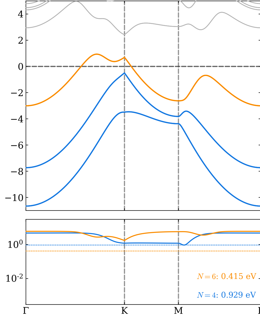
(b) 1H- \beta -beryllene: Z_2 = 0/0 (WCC) N = 4/6
