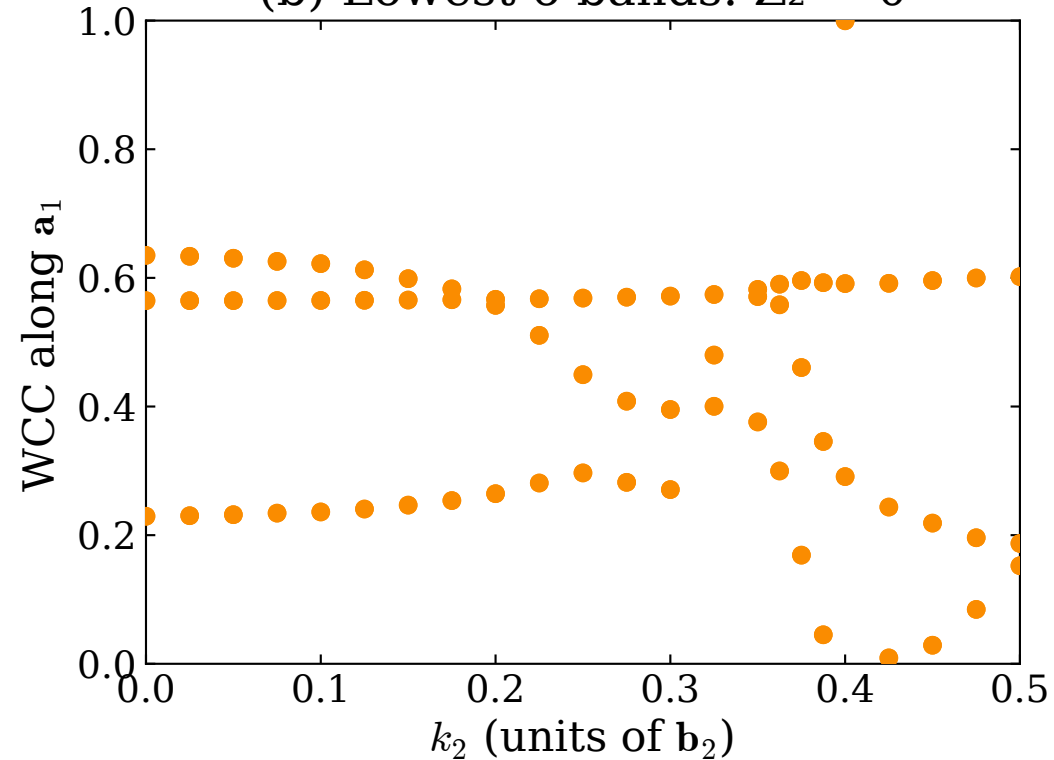
(b) Lowest 6 bands: Z_2 = 0
