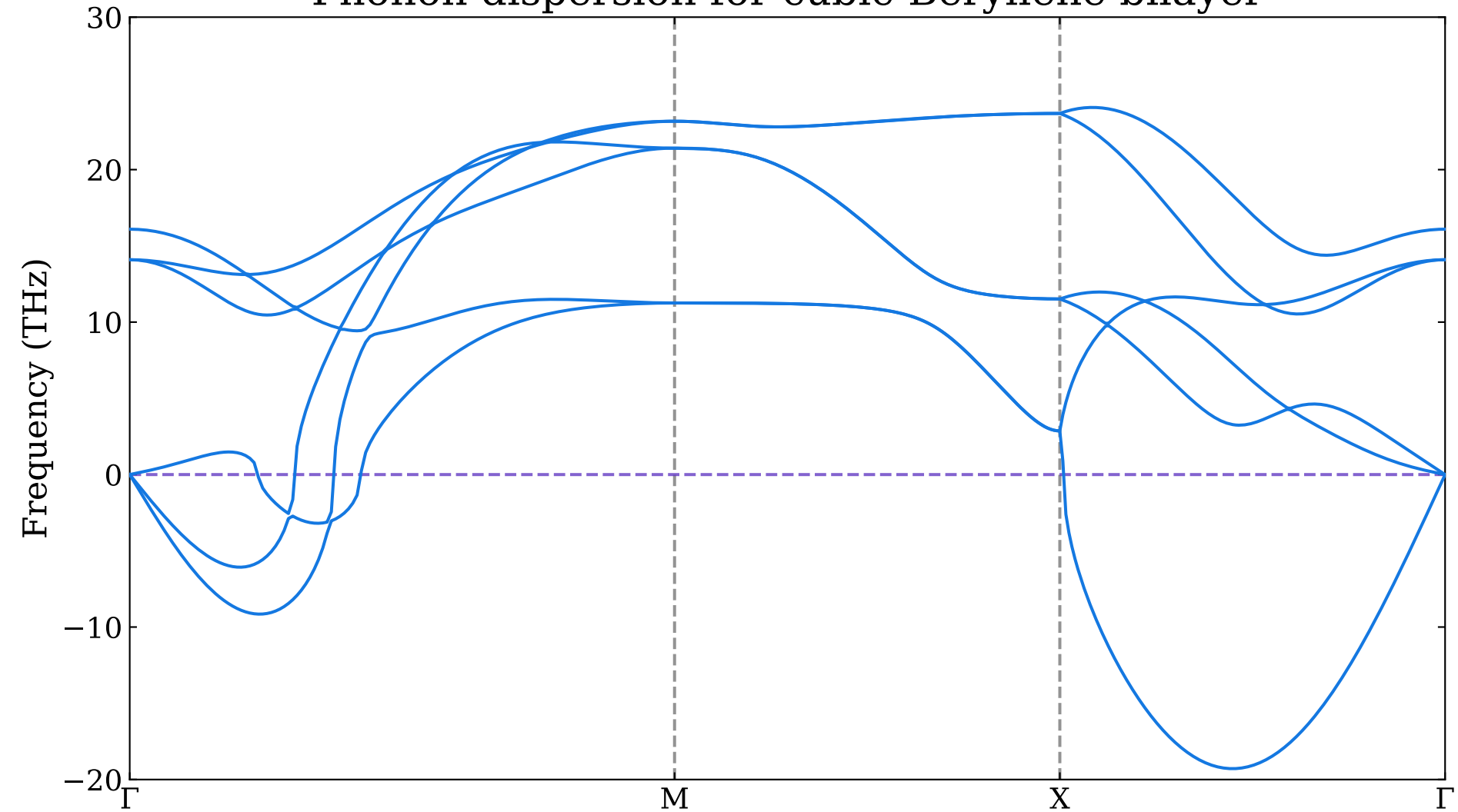
Phonon dispersion for cubic-Beryllene bilayer
