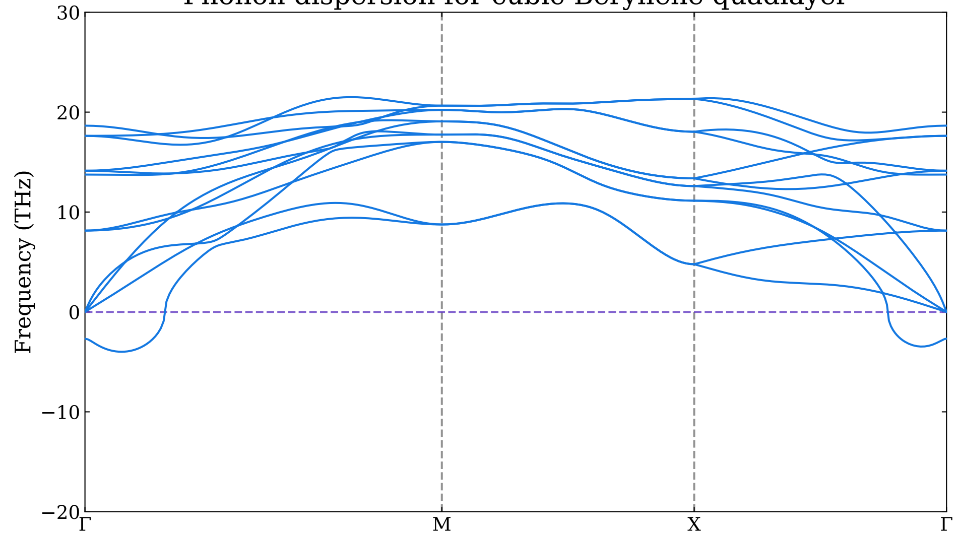
Phonon dispersion for cubic-Beryllene quadlayer
