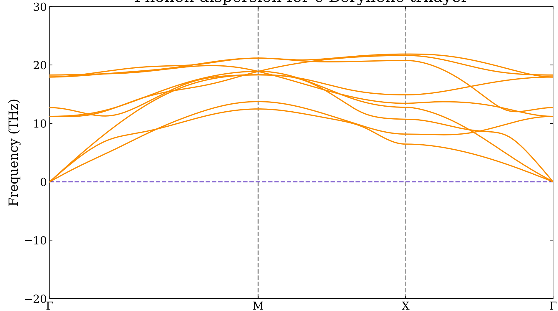
Phonon dispersion for c-Beryllene trilayer
