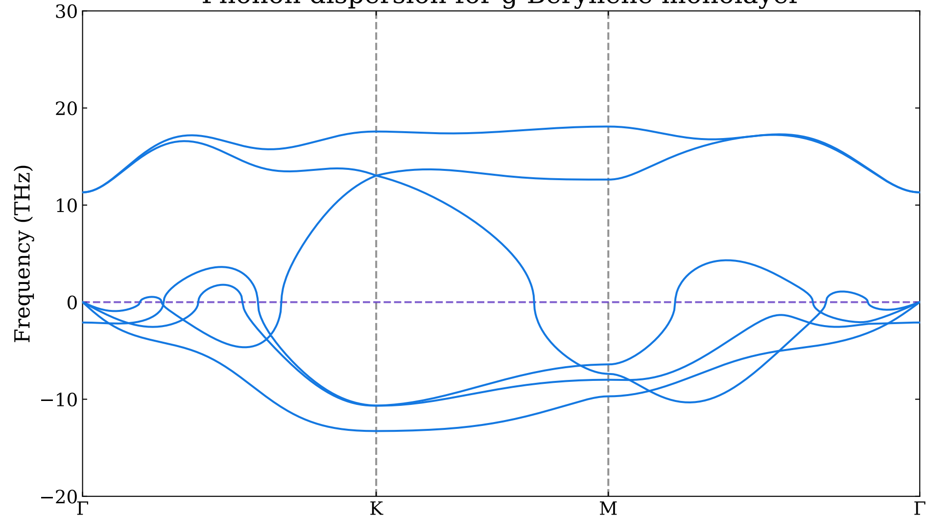
Phonon dispersion for g-Beryllene monolayer
