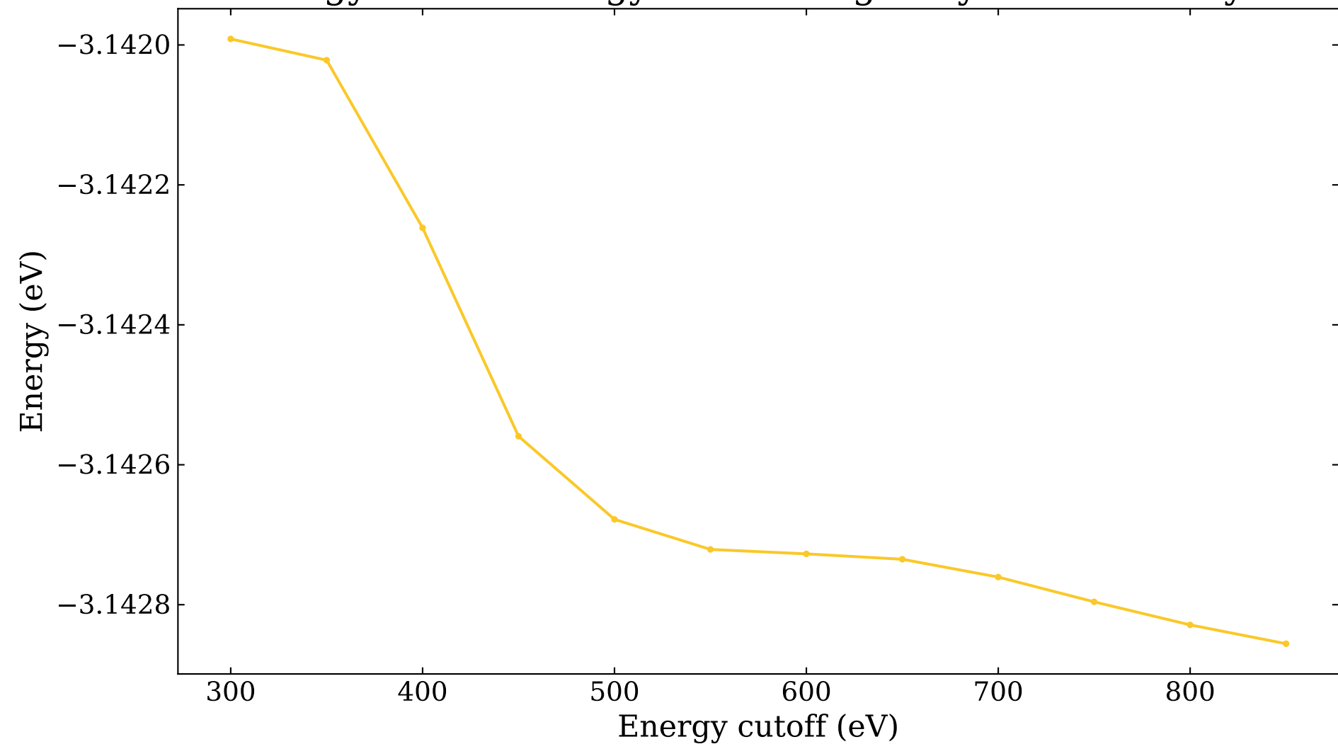
Energy versus energy cutoff for g-Beryllene monolayer
