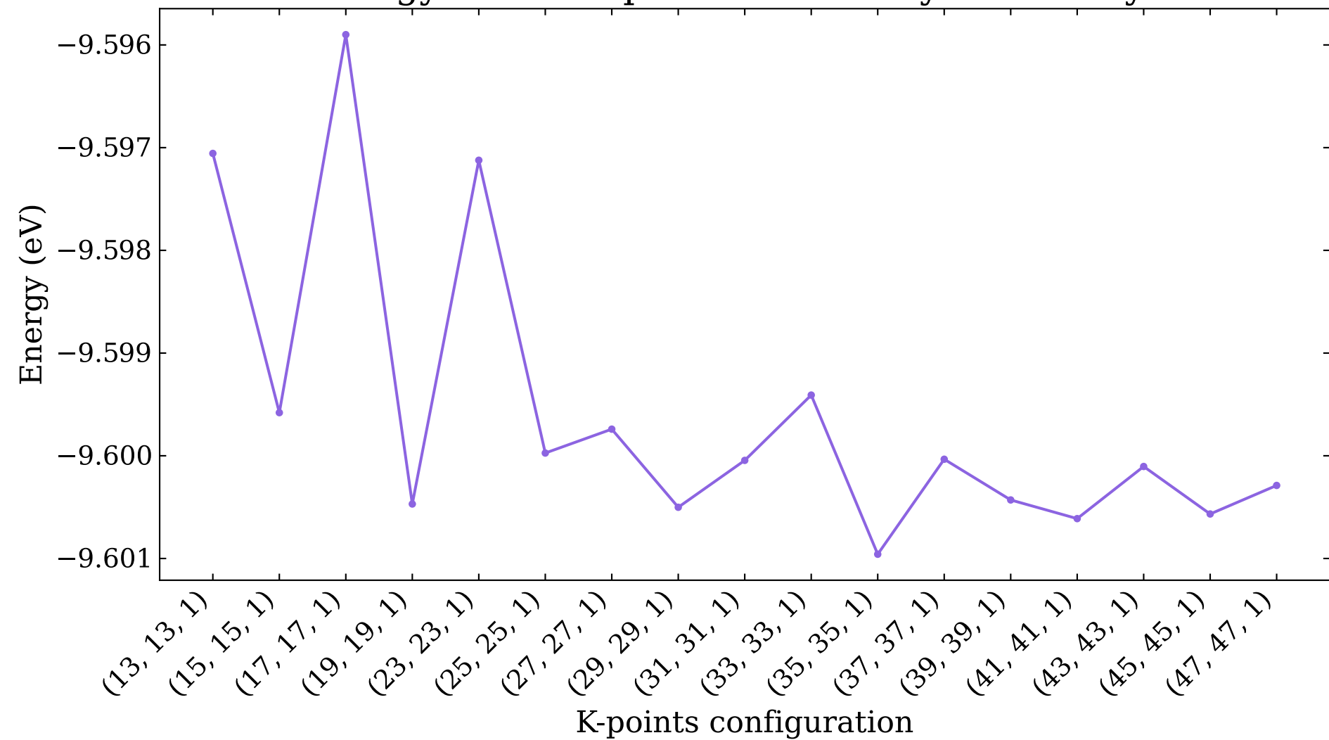
Energy versus k-points for c-Beryllene trilayer
