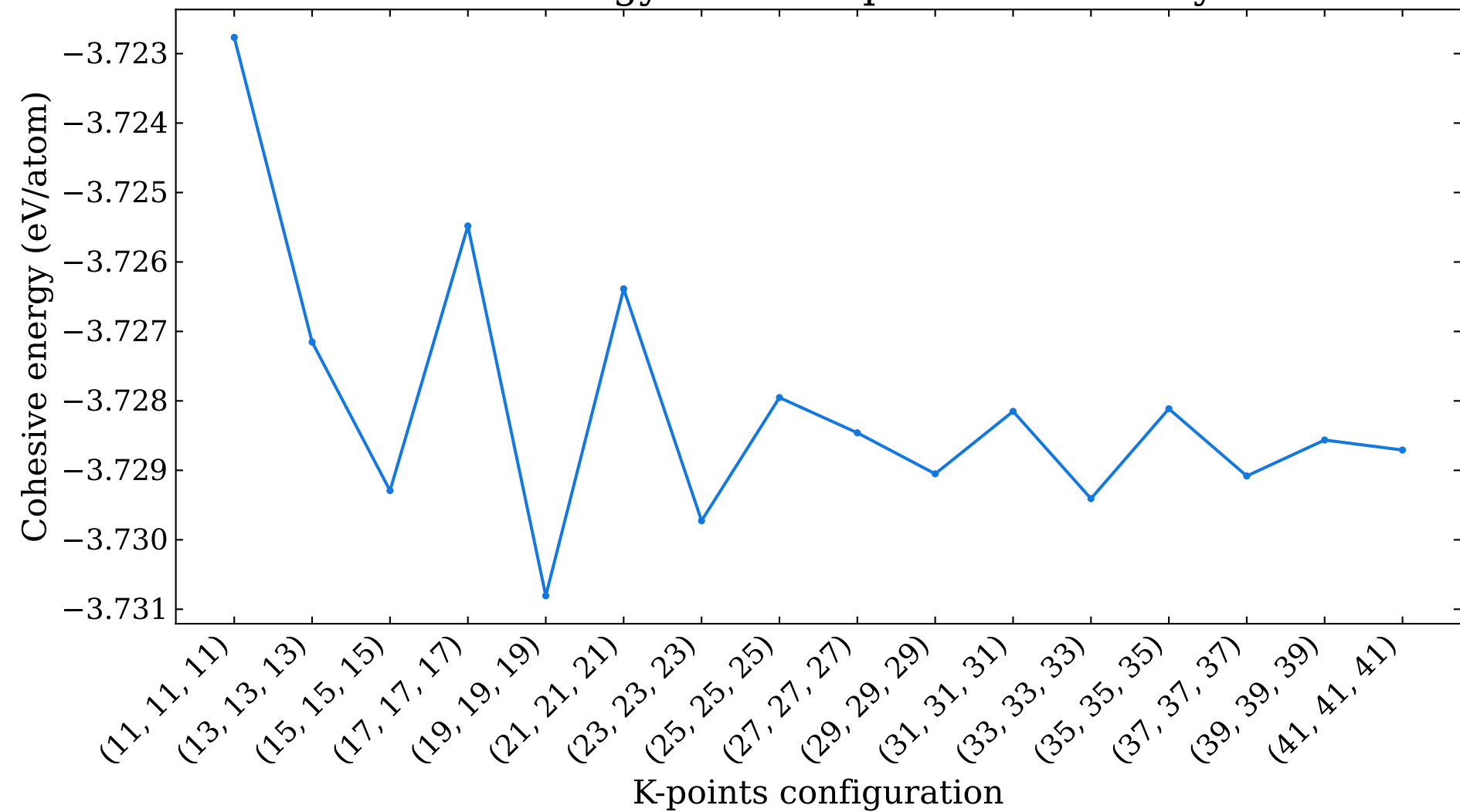
Cohesive energy versus k-points for \alpha -Beryllium
