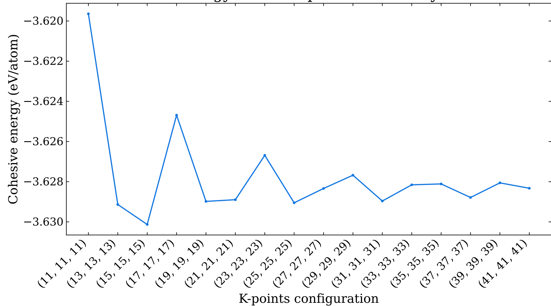
Cohesive energy versus k-points for c-Beryllene bulk
