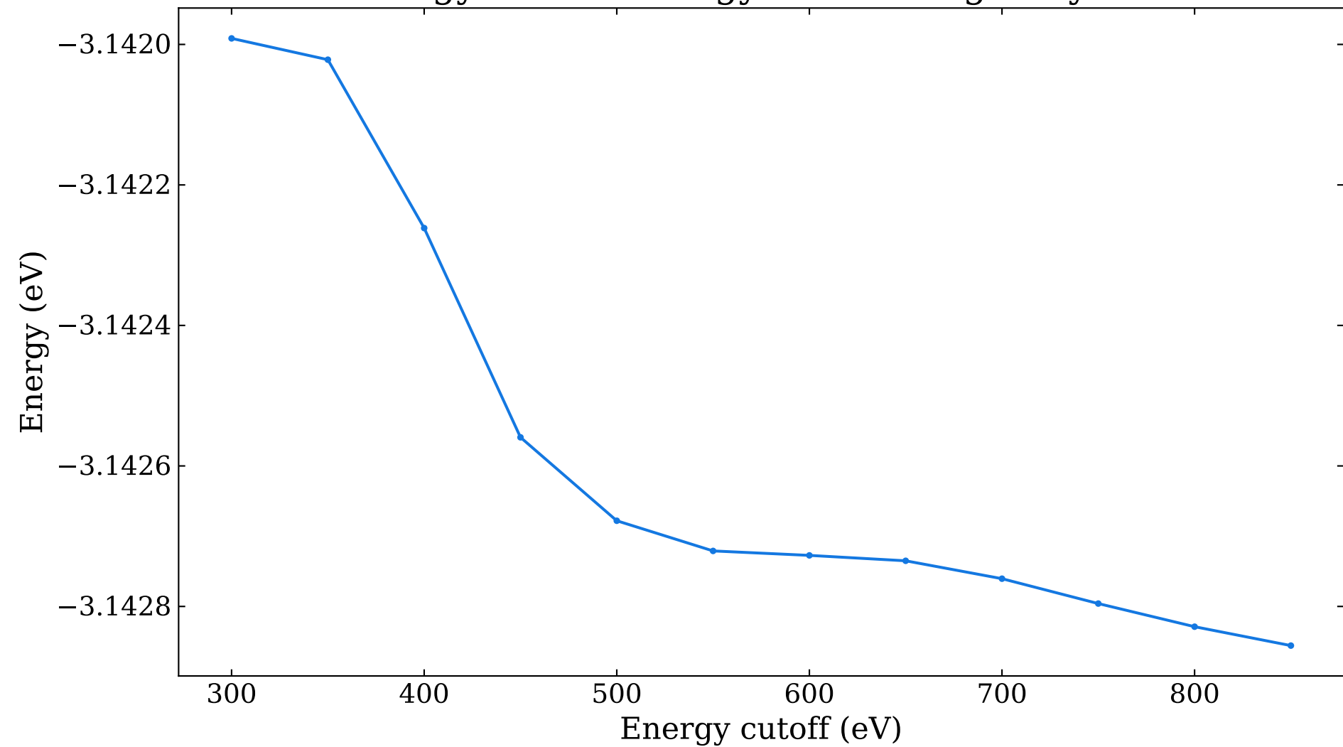
Energy versus energy cutoff for g-Beryllene
