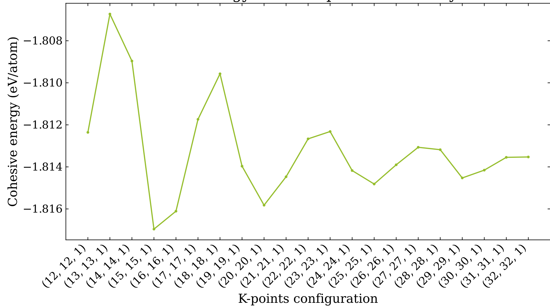
Cohesive energy versus k-points for c-Beryllene
