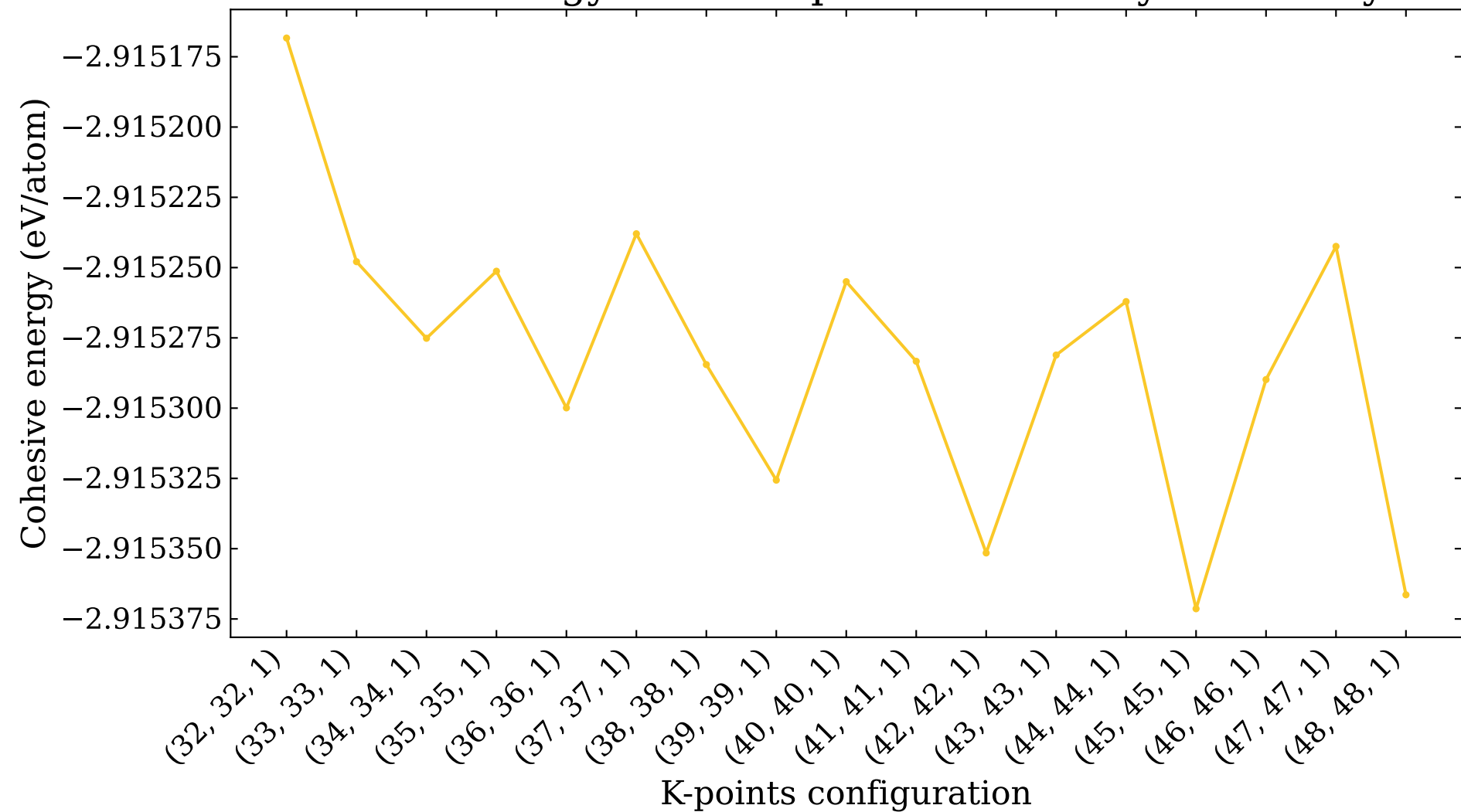
Cohesive energy versus k-points for c-Beryllene trilayer
