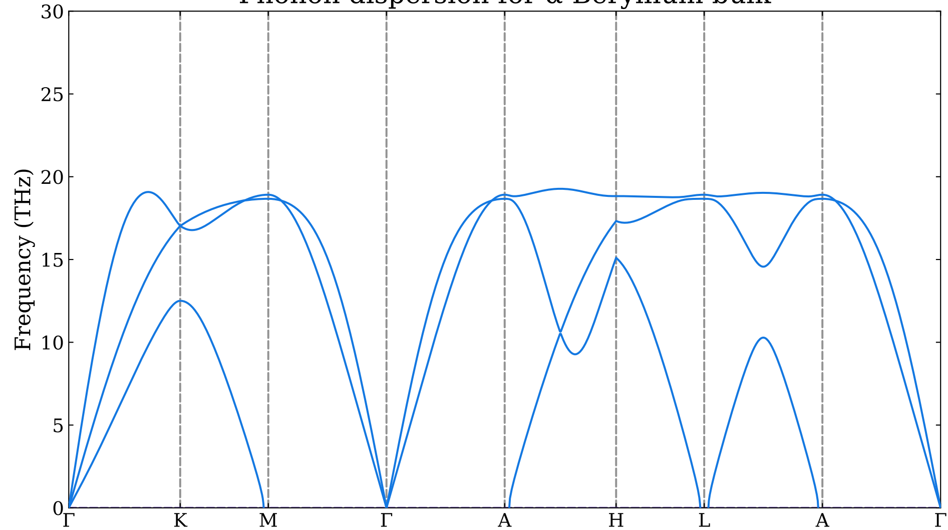
Phonon dispersion for \alpha -Beryllium bulk
