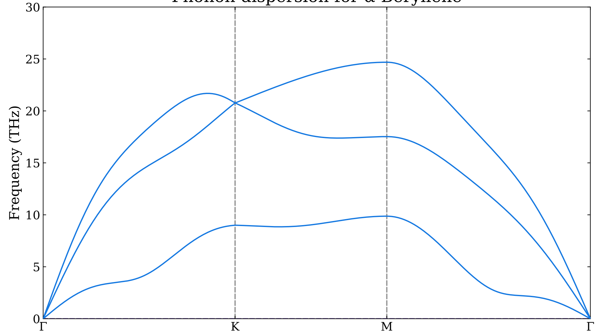
Phonon dispersion for \alpha -Beryllene
