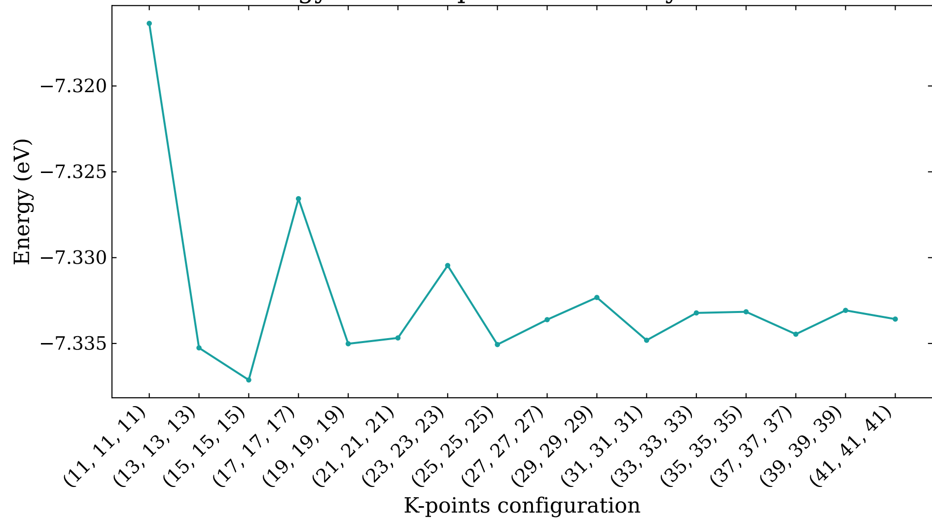
Energy versus k-points for c-Beryllene bulk
