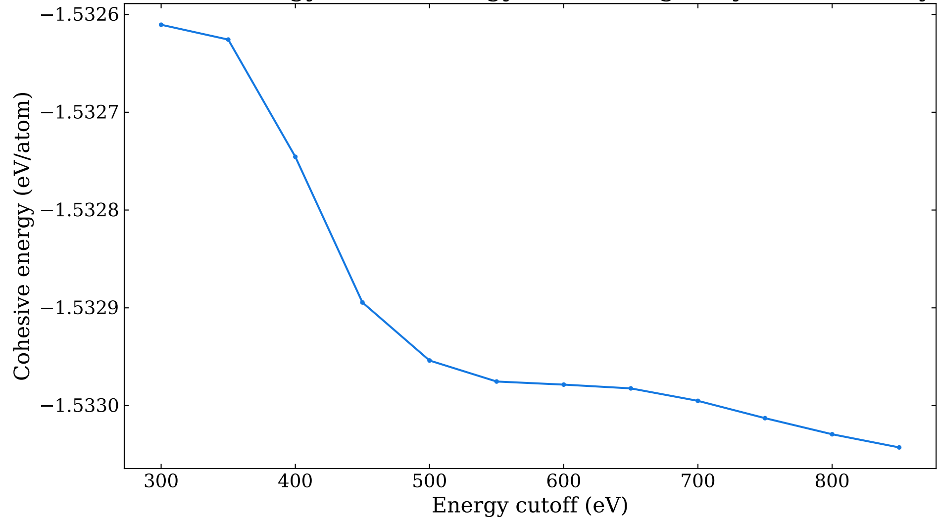
Cohesive energy versus energy cutoff for g-Beryllene monolaye
