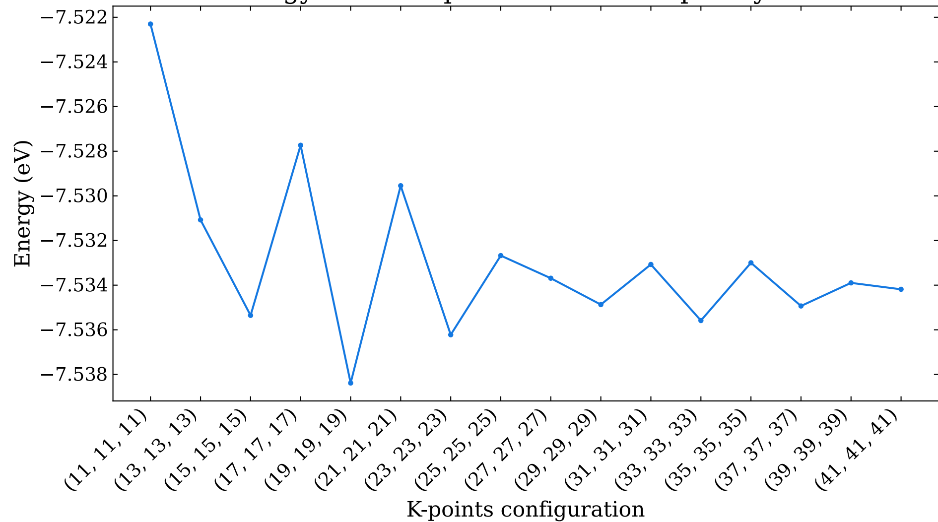
Energy versus k-points for bulk hcp Beryllene
