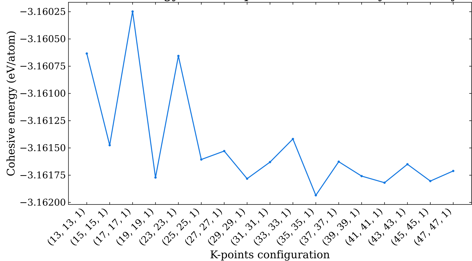
Cohesive energy versus k-points for cubic-Beryllene trilayer
