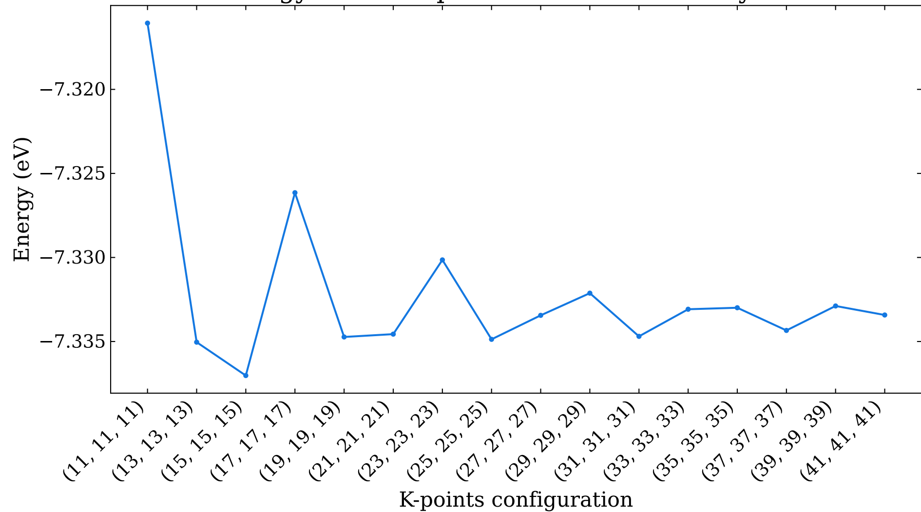
Energy versus k-points for bulk bcc Beryllene
