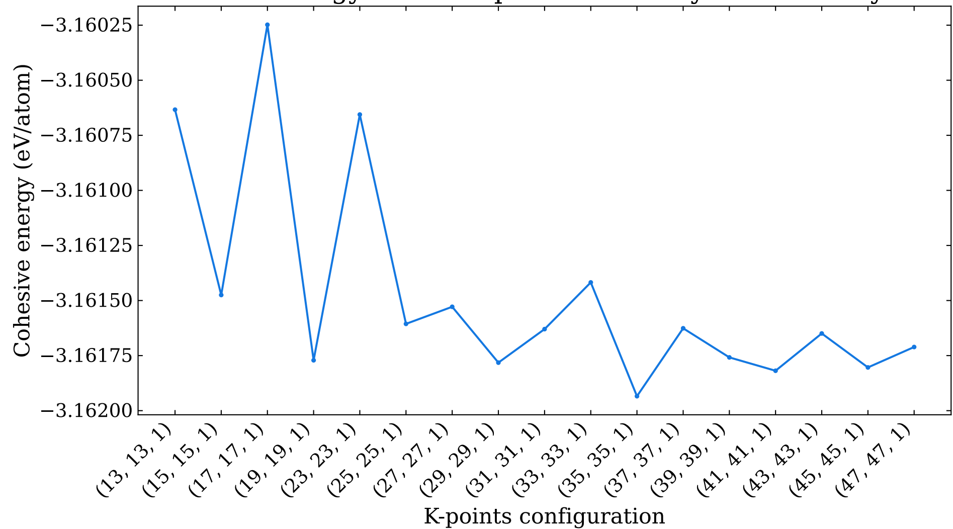
Cohesive energy versus k-points for trilayer cubic beryllene
