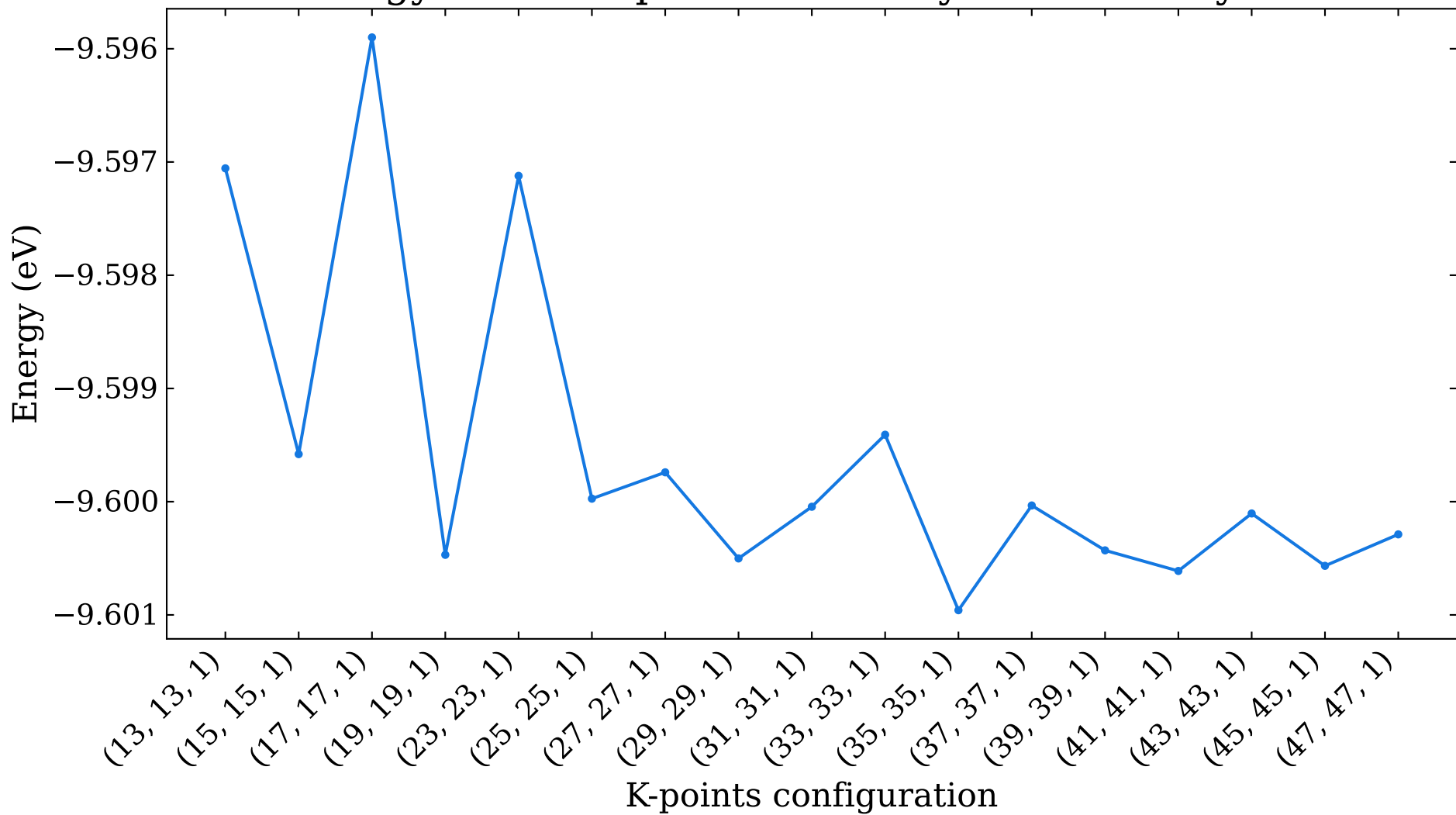
Energy versus k-points for trilayer cubic beryllene
