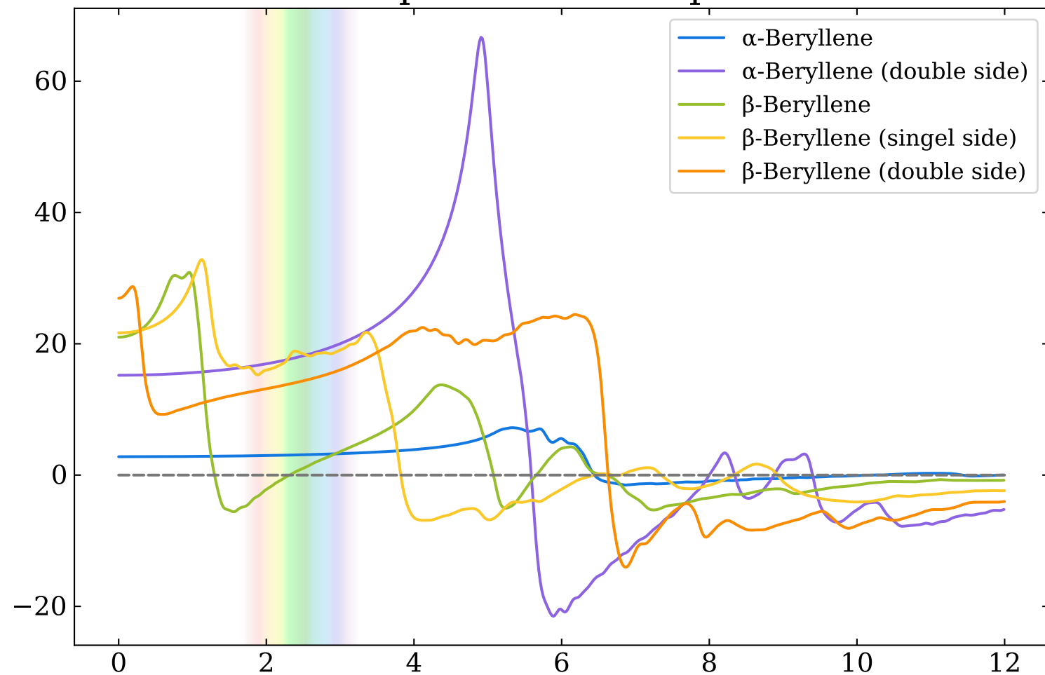
Imaginary part for xx-component
