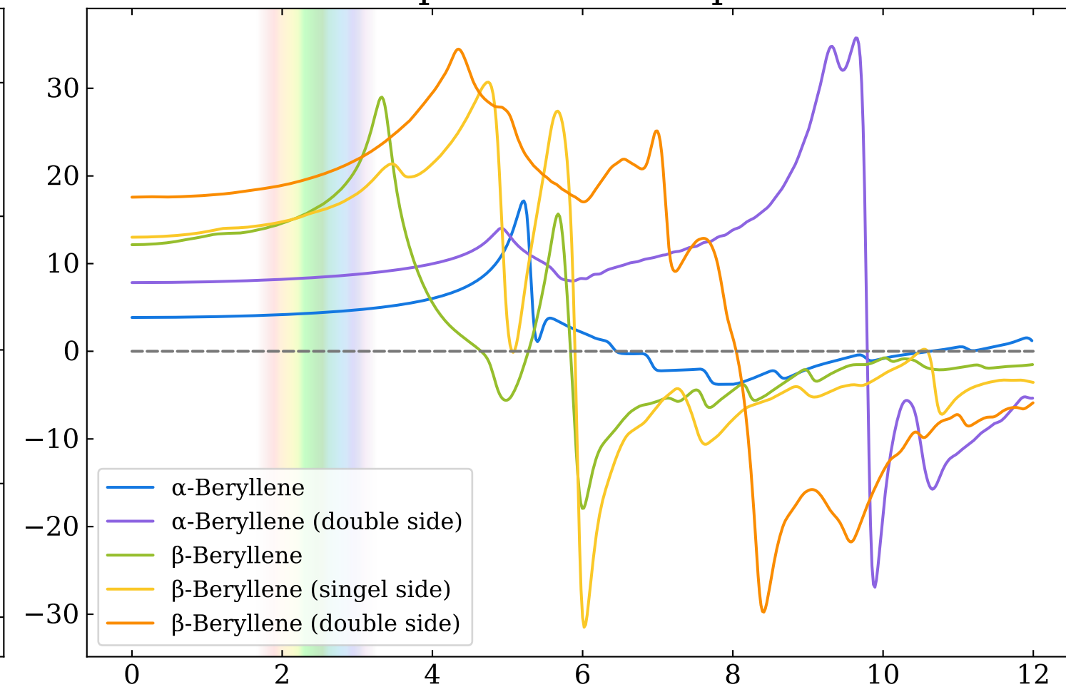
Imaginary part for zz-component
