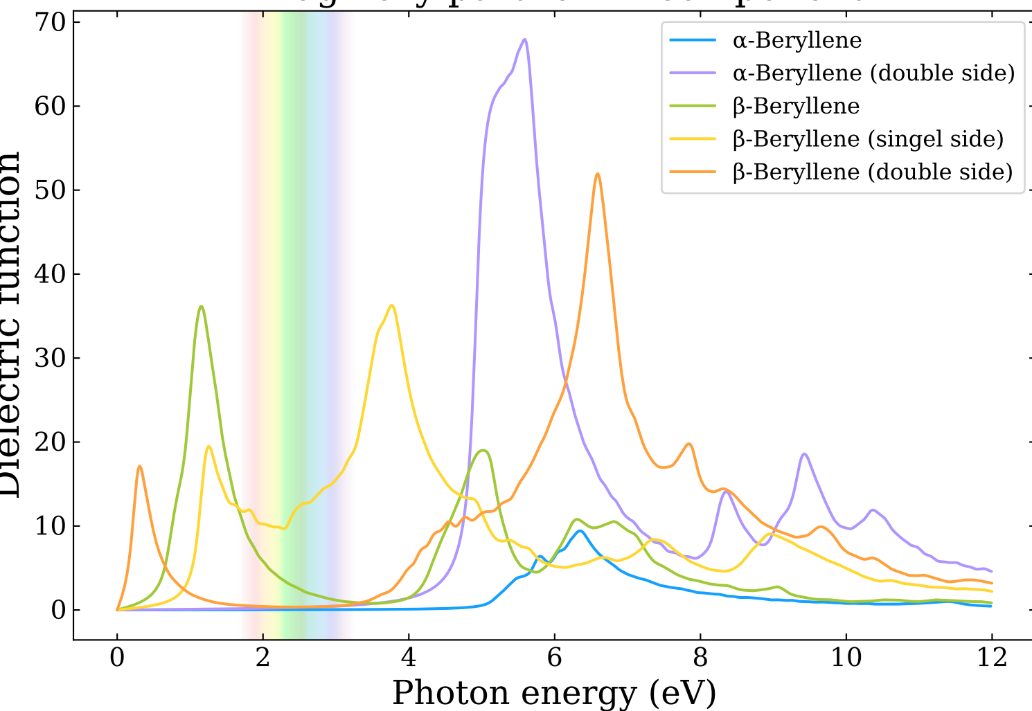
Imaginary part for xx-component
