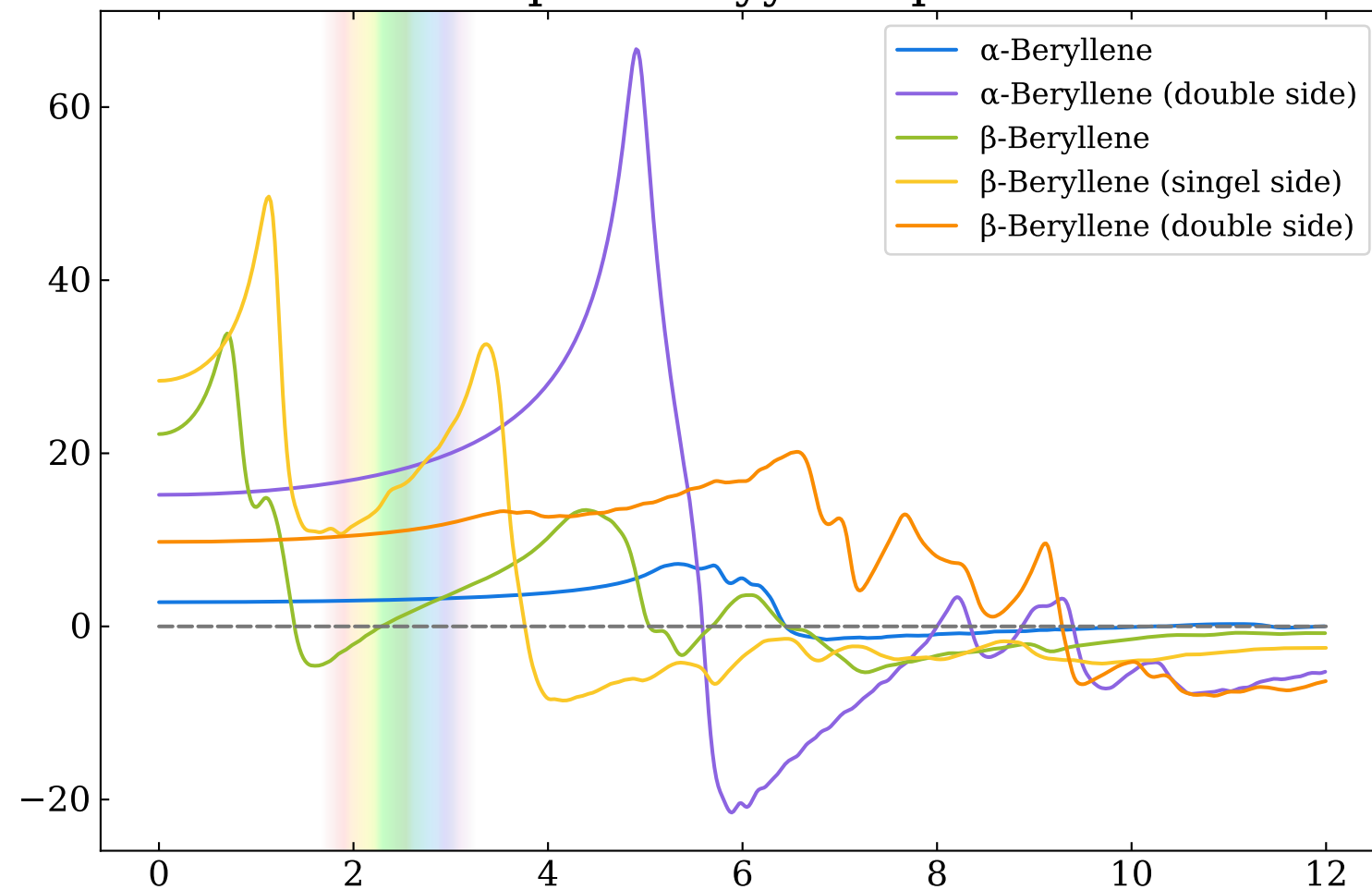
Imaginary part for yy-component
