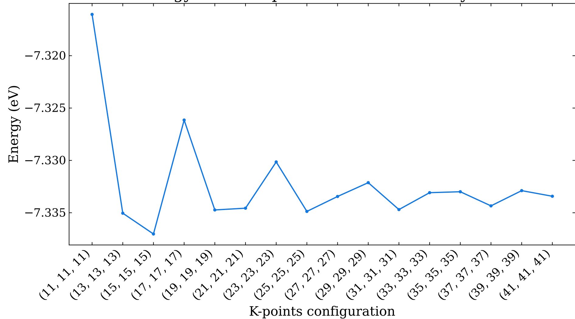
Energy versus k-points for bulk bcc Beryllium
