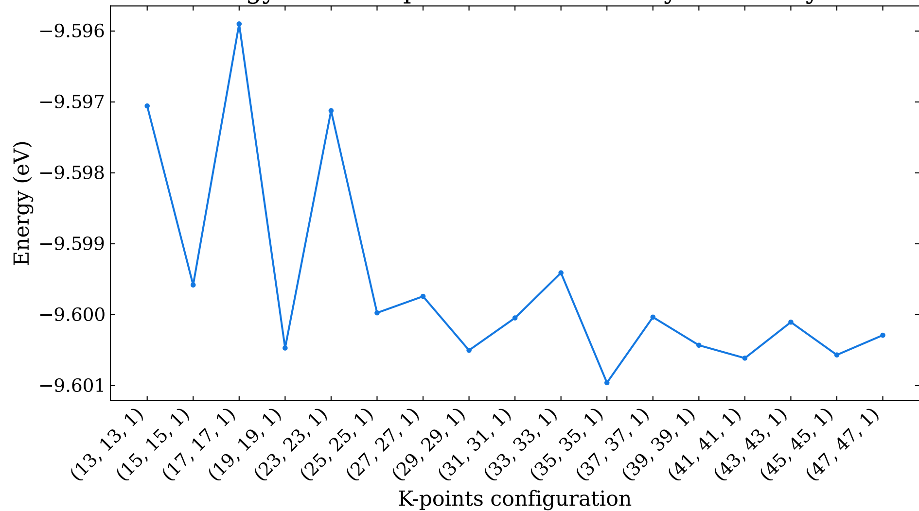
Energy versus k-points for cubic Beryllene trilayer
