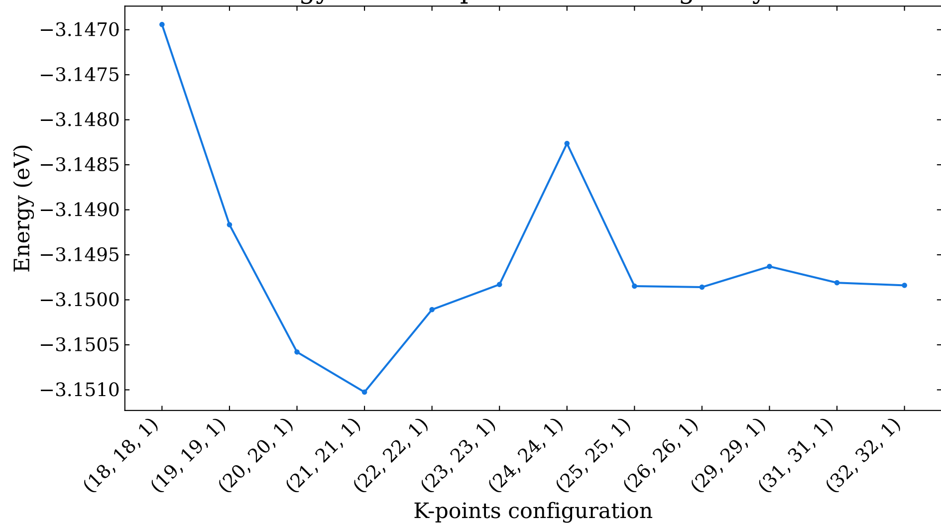
Energy versus k-points mesh for g-Beryllene
