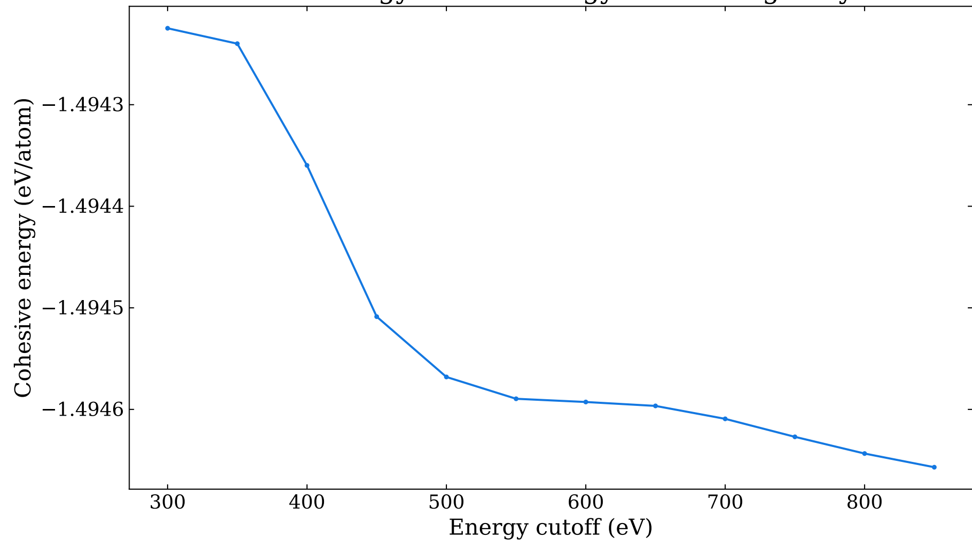
Cohesive energy versus energy cutoff for g-Beryllene
