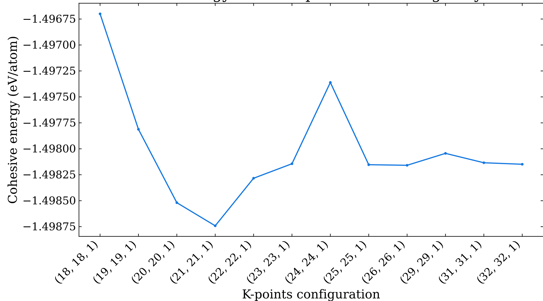
Cohesive energy versus k-points mesh for g-Beryllene
