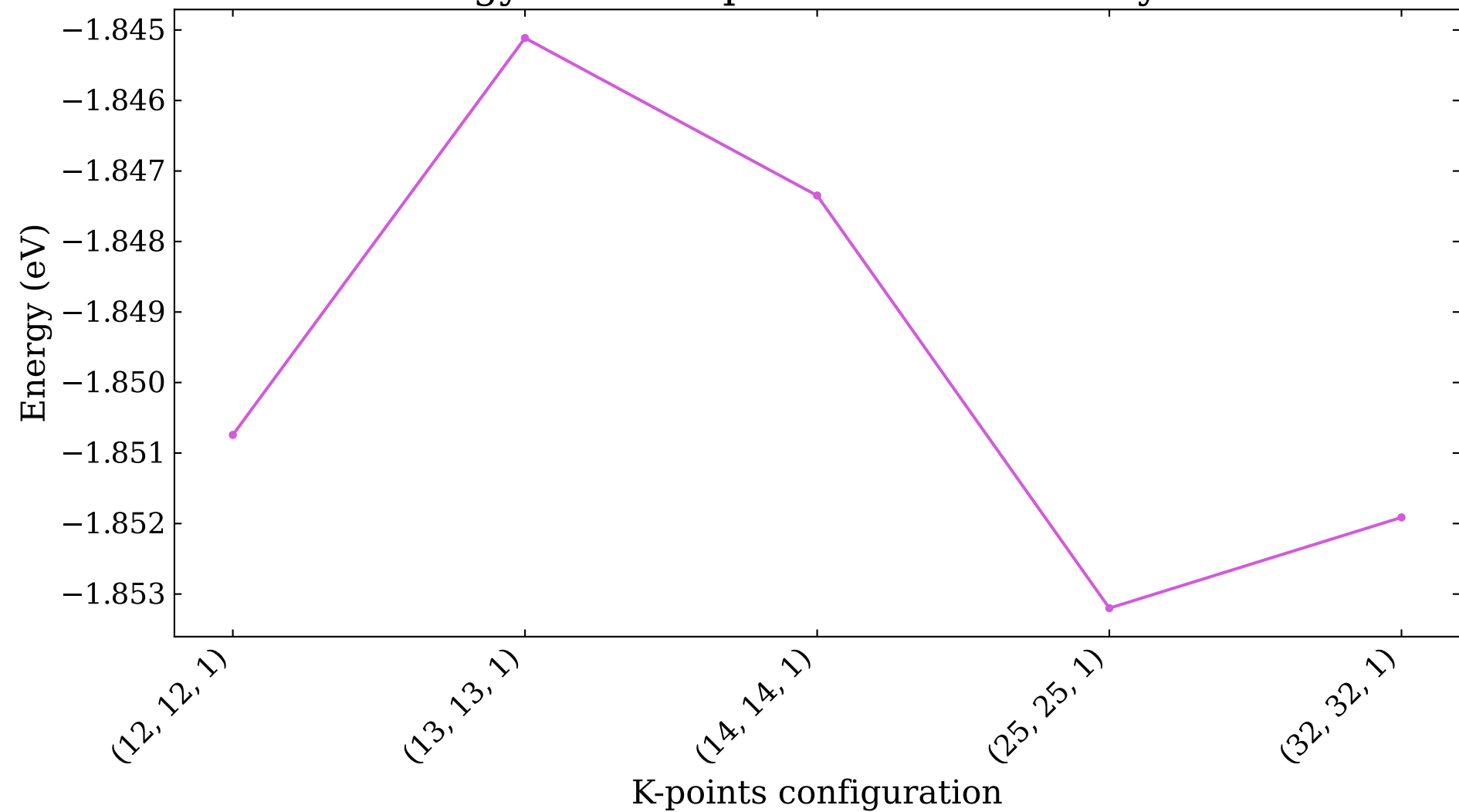
Energy versus k-points for cubic-Beryllene
