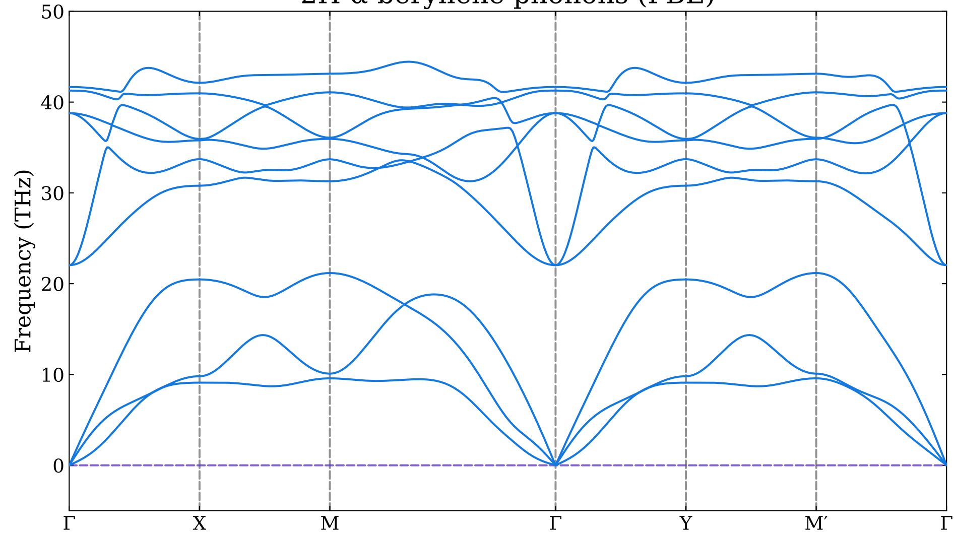
2H- \alpha -beryllene phonons (PBE)
