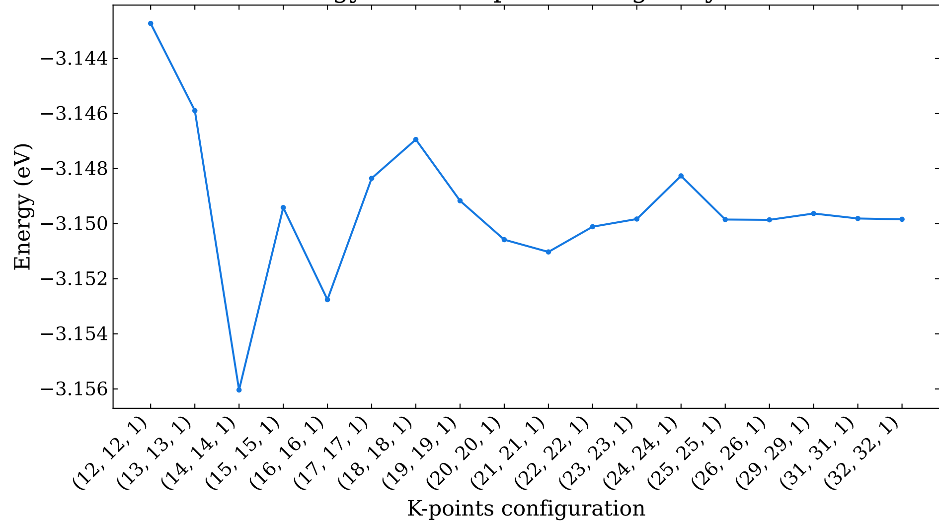
Energy versus k-points for g-Beryllene
