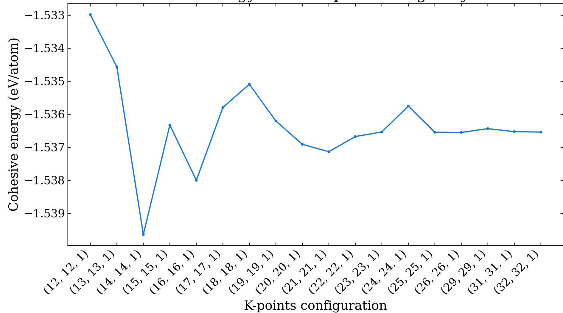
Cohesive energy versus k-points for g-Beryllene
