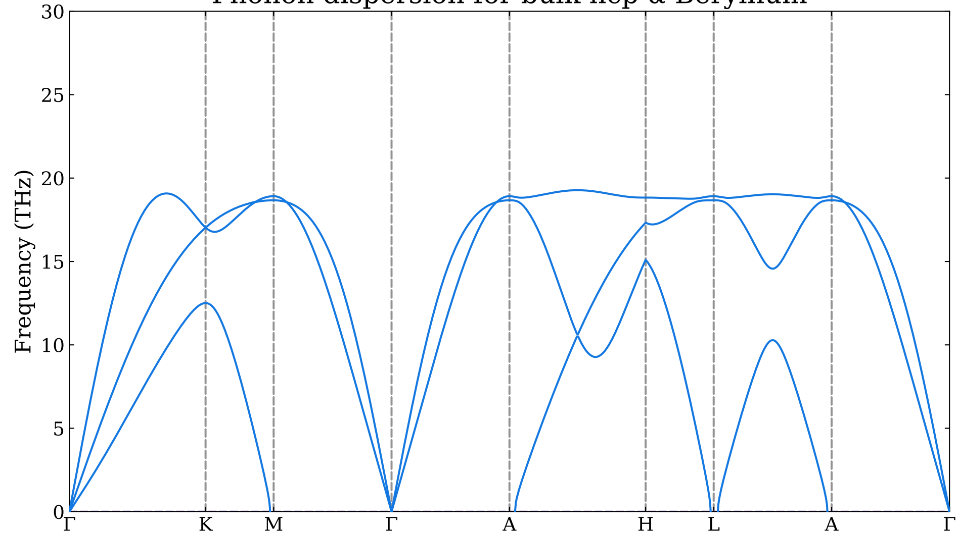
Phonon dispersion for bulk hcp \alpha -Beryllium
