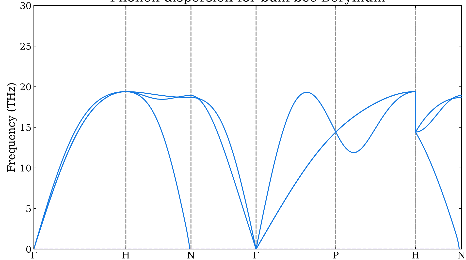
Phonon dispersion for bulk bcc Beryllium
