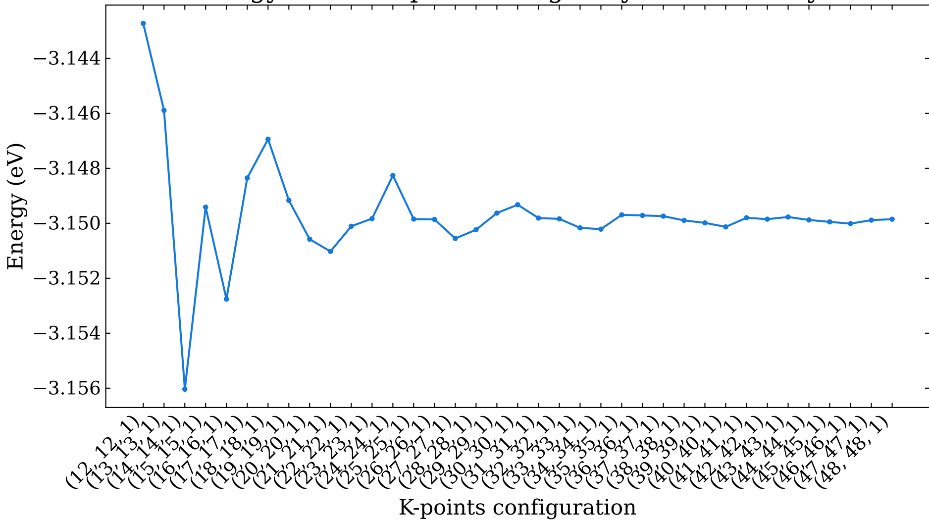
Energy versus k-points for g-Beryllene monolayer
