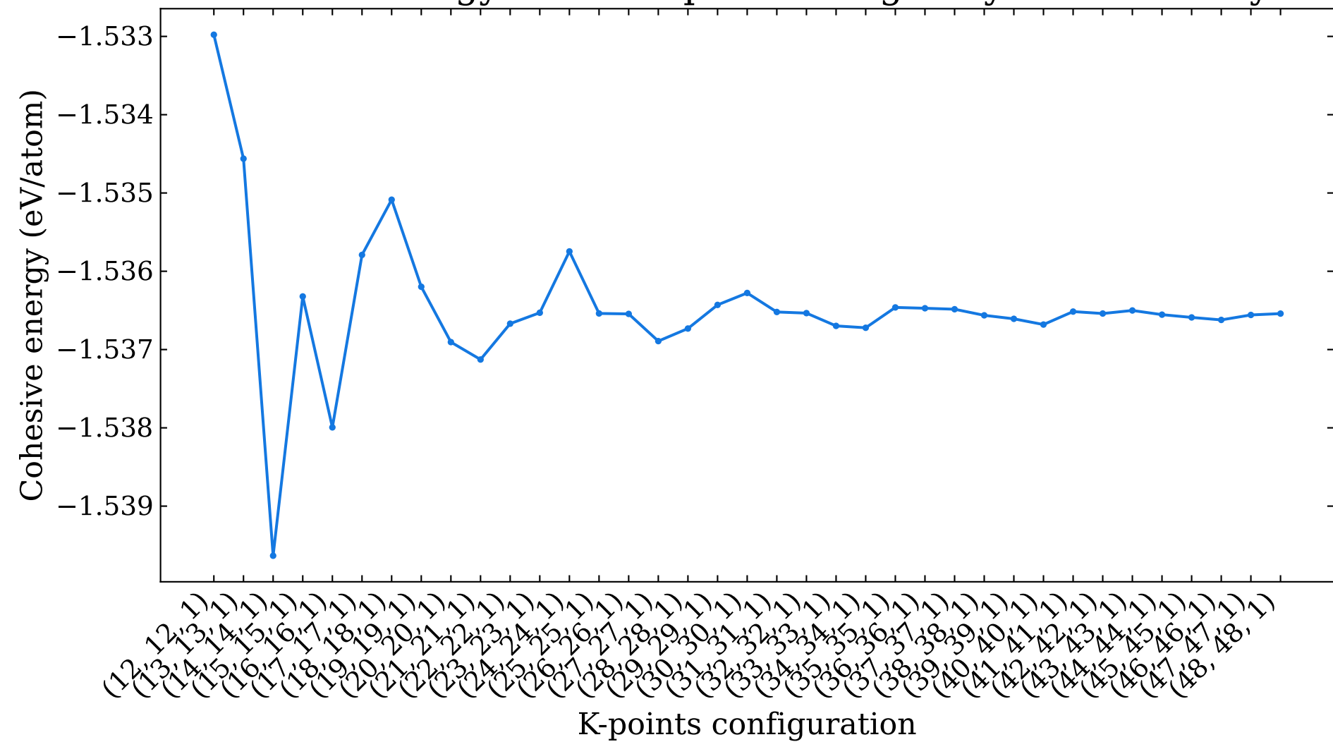
Cohesive energy versus k-points for g-Beryllene monolayer
