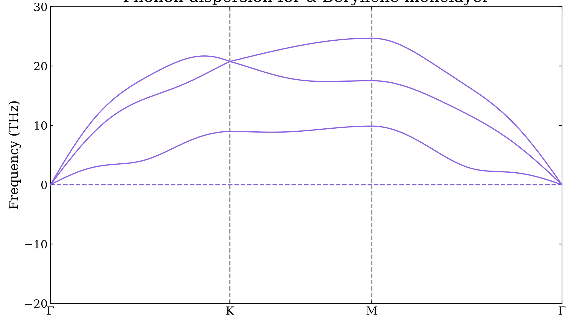
Phonon dispersion for \alpha -Beryllene monolayer
