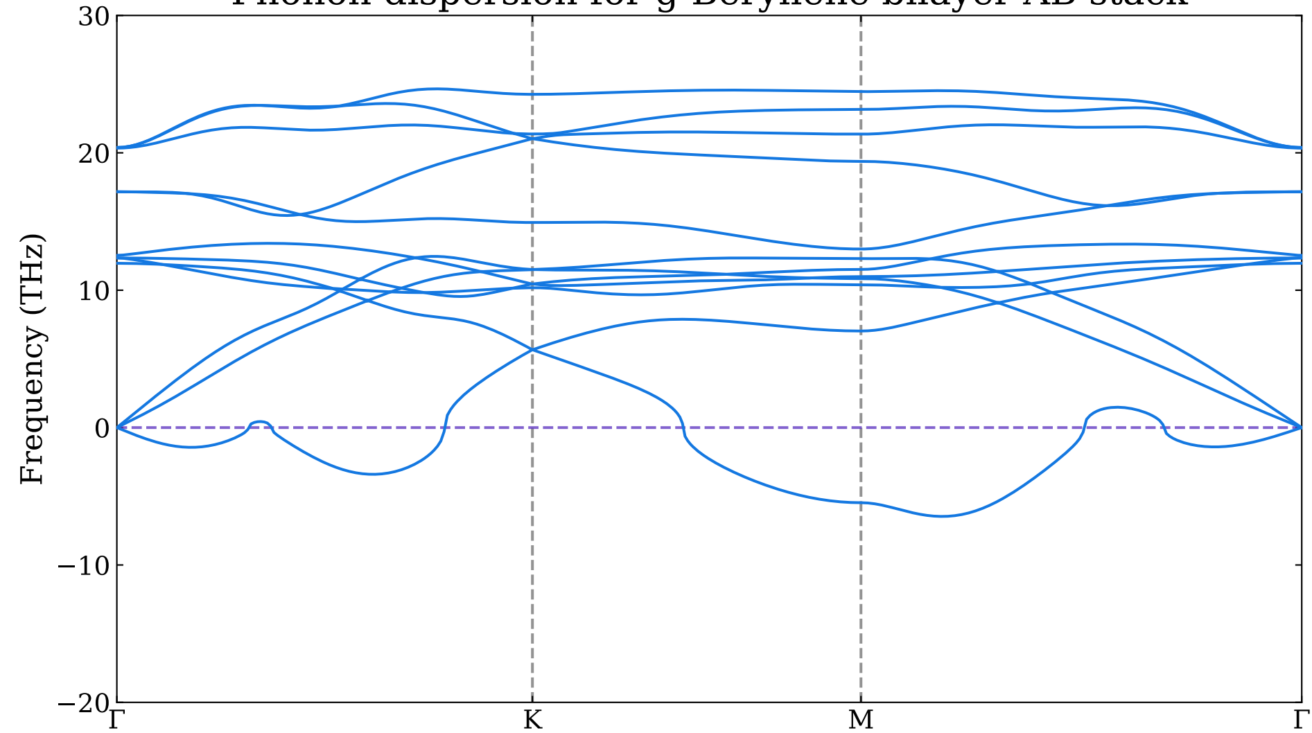
Phonon dispersion for g-Beryllene bilayer AB stack
