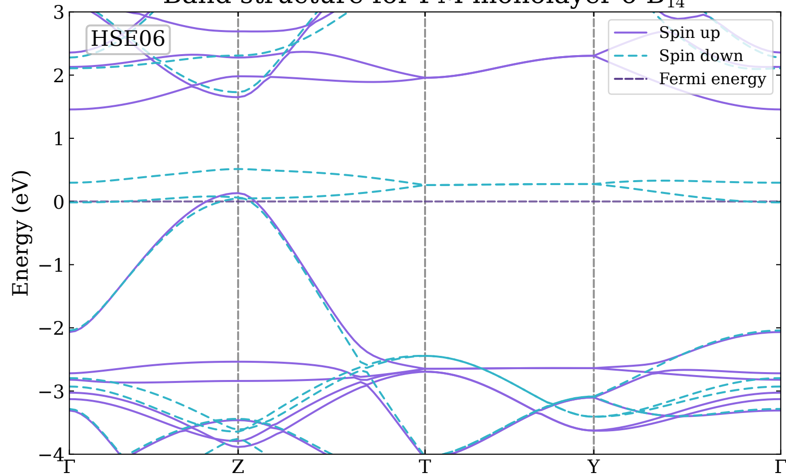
Band structure for FM monolayer o-B 14
