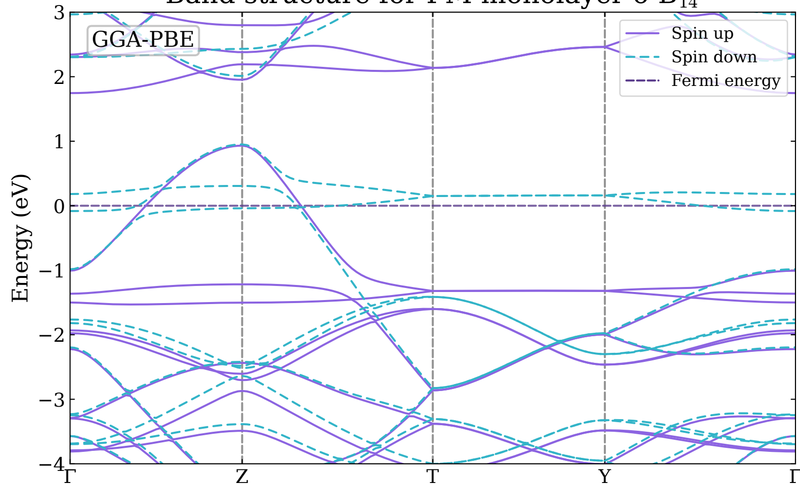
Band structure for FM monolayer o-B 14
