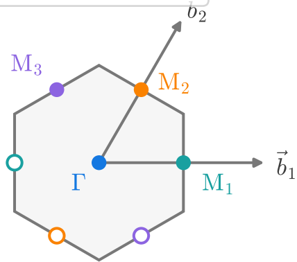
(a) Triangular lattice
