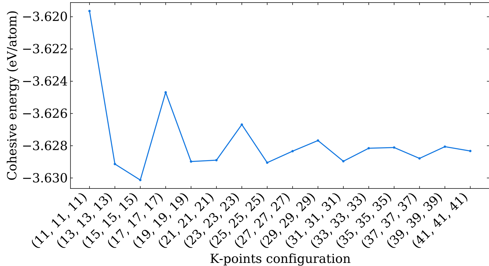
Cohesive energy versus k-points for bulk bcc beryllium
