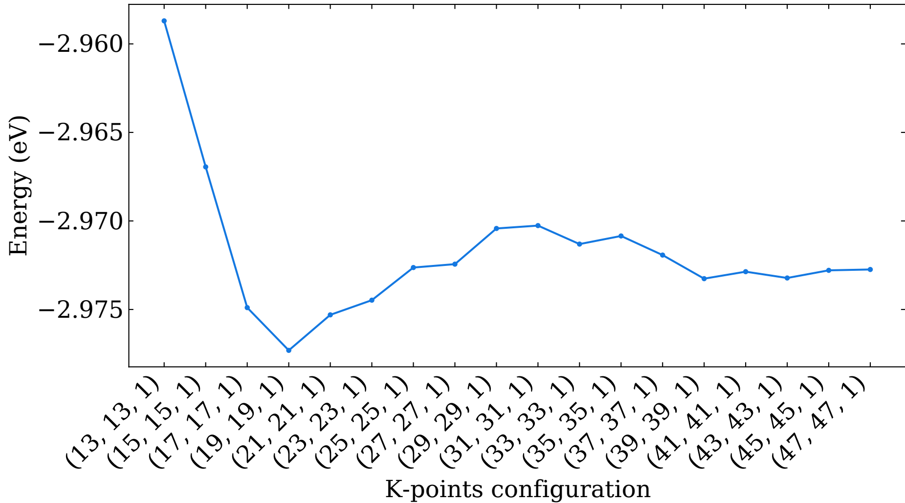
Energy versus k-points for \alpha -beryllene
