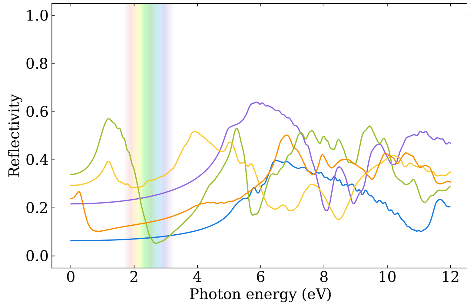
zz-component
