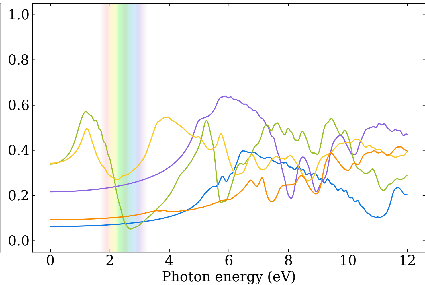
yy-component
