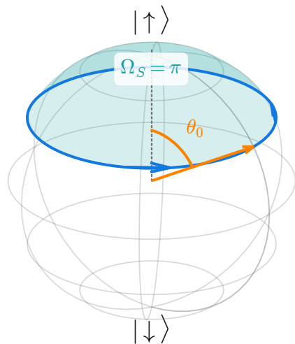
(a) A loop on the state sphere
