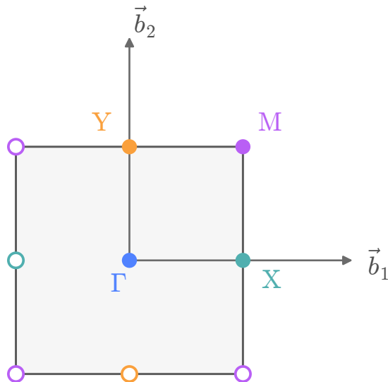
(b) Square lattice
