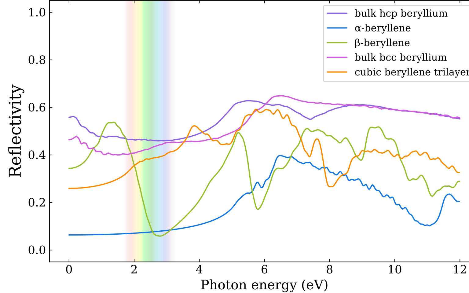
xx-component
