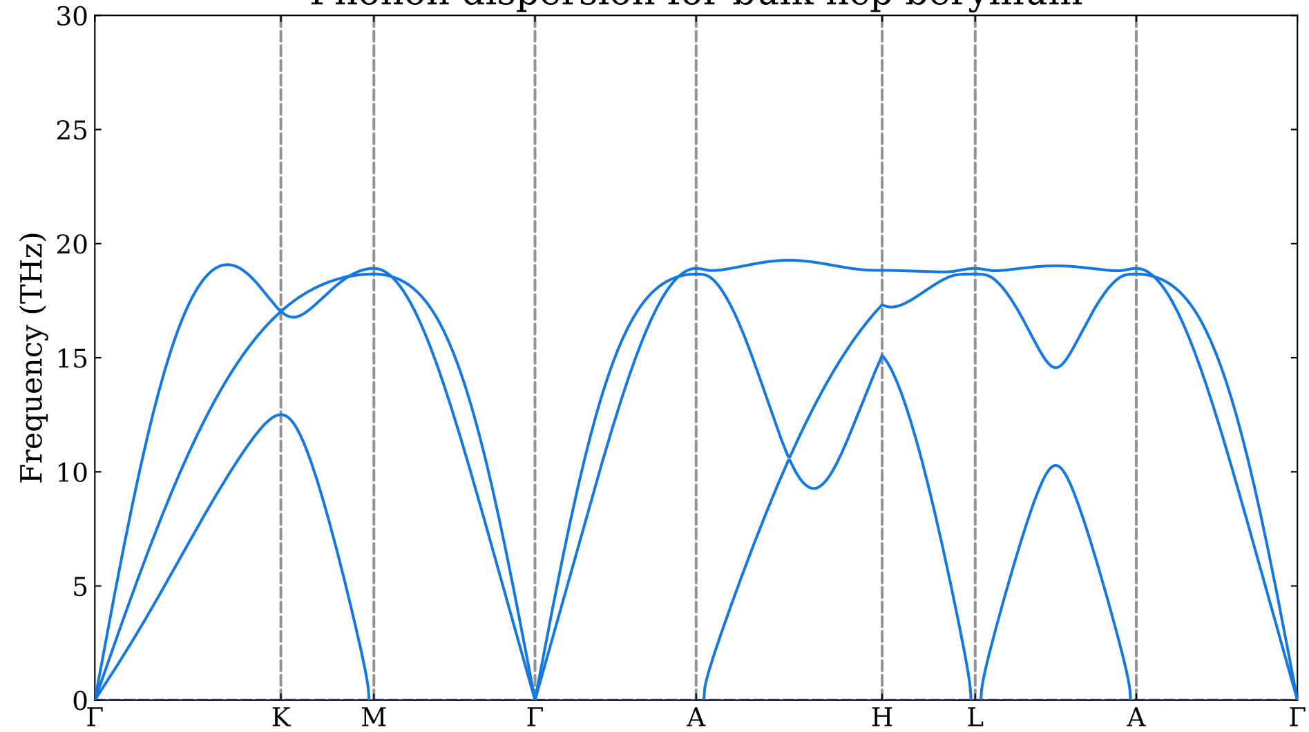
Phonon dispersion for bulk hcp beryllium
