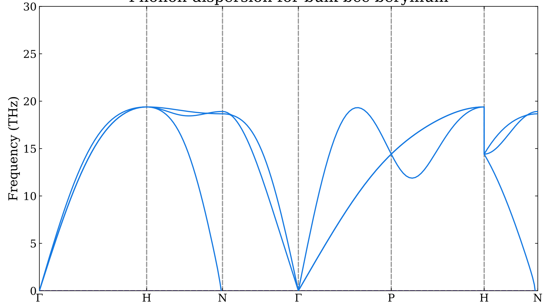
Phonon dispersion for bulk bcc beryllium
