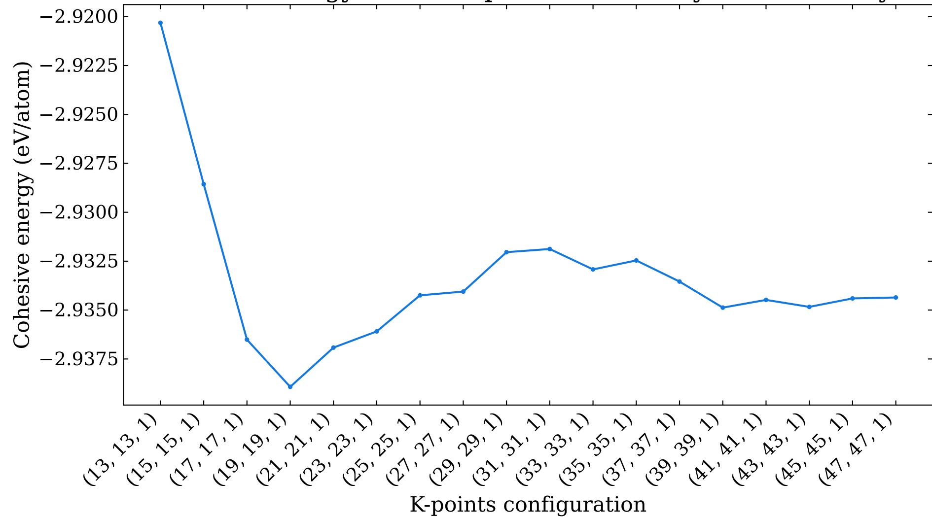
Cohesive energy versus k-points for \alpha -beryllene monolayer
